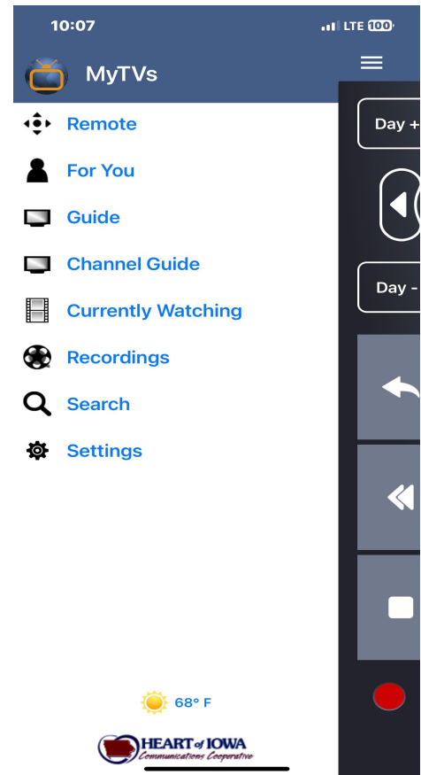
Figure 1-2 MyTVs Menu
